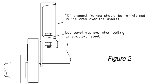
Top Mount Installation
